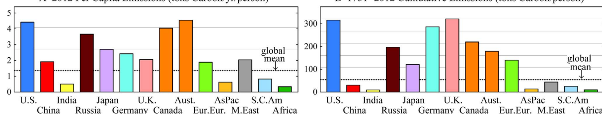
Figure 12. Per capita fossil fuel CO 2 emissions. Countries, regions and data sources are the same as in Fig. 11. Horizontal lines are the global mean and multiples of the global mean. doi:10.1371/journal.pone.0081648.g012
