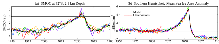
Figure 27. (a) SMOC, the global meridional overturning circulation at 72° S, in climate model runs including freshwater injection around Antarctica at a rate 720 Gt yr -1 in 2011, increasing with a 10 year doubling time, and half that amount around Greenland. SMOC diagnostic includes only the mean (Eulerian) term. (b) Annual-mean Southern Hemisphere sea ice area anomaly (relative to 1979–2000) in the five runs.
