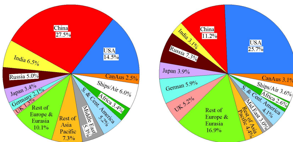
(a) 2013 Annual Emissions (9.9 GtC/yr) (b) 1751–2013 Cumulative Emis. (394 GtC)
